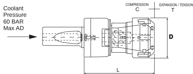
Style A — Straight Shank
