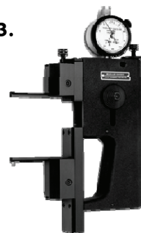
3. Model 179 with 1400 carbide ball tips to check internal diameter of parts with spherical radius. Also checks pitch diameter of splines and gears. See 1400 brochure.
