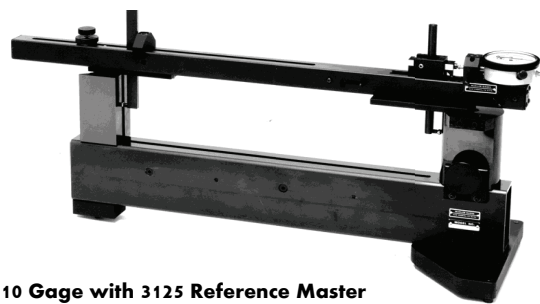
2910 Gage with 3125 Reference Master
