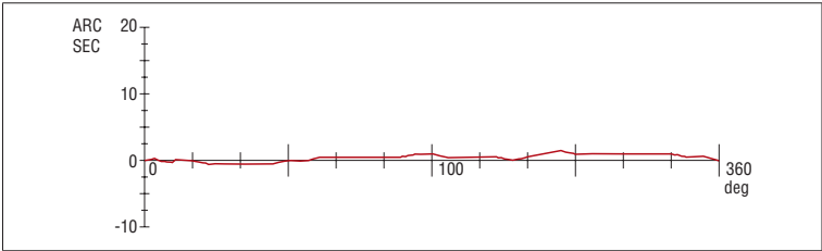
Example of indexing accuracy measurement with encoders or scales.
