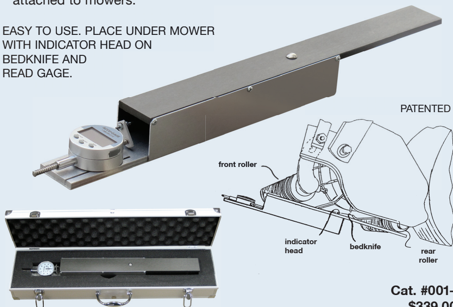
ACCU-GAGE II SUPPLIED IN ALUMINUM CASE.
